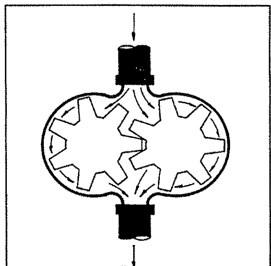
Figure 3. Gear Pump
