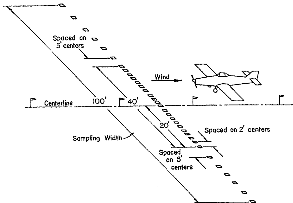
Figure 11. Pattern evaluation layout
