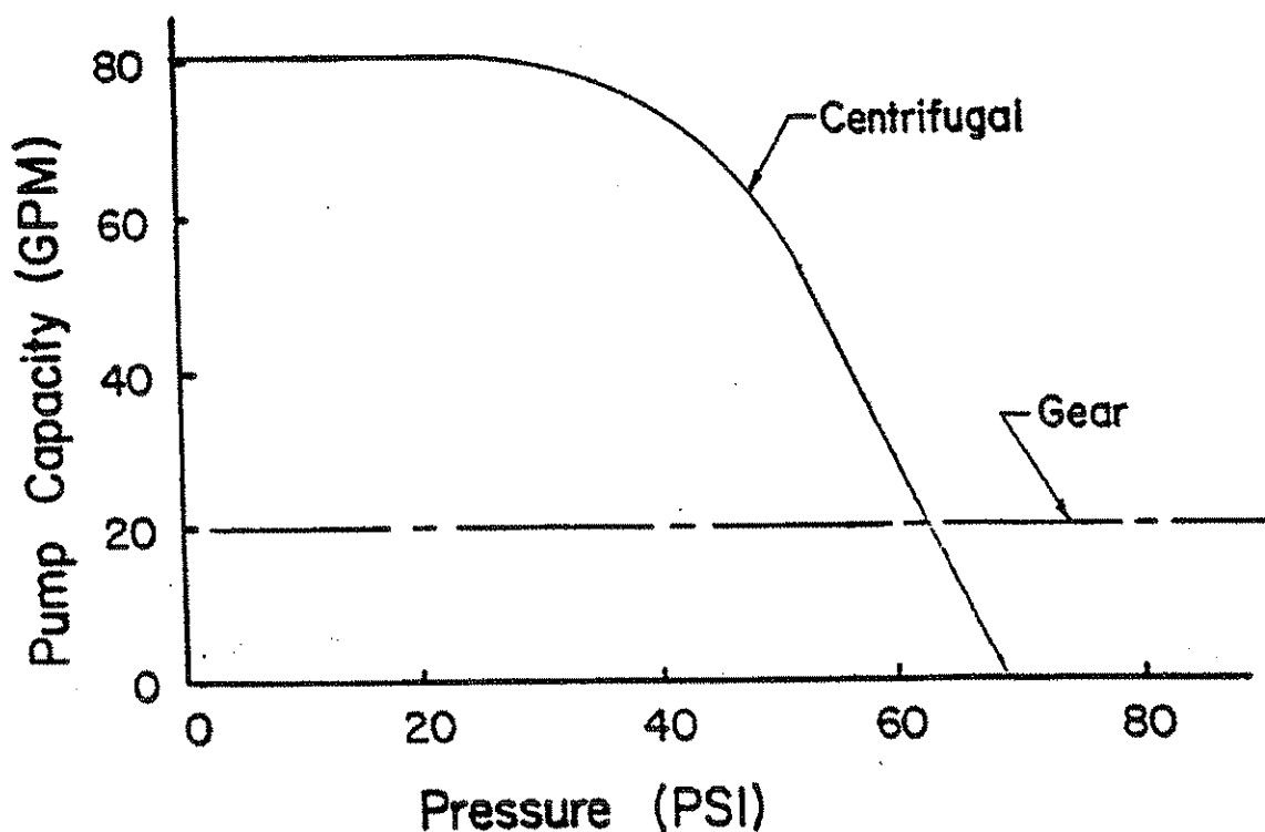
Figure 4. Pump performance curves for centrifugal and gear pumps.
