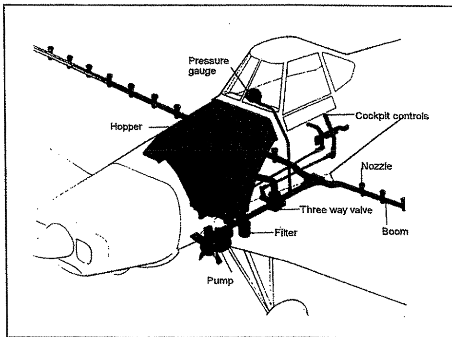
Figure 1. Liquid dispersal system for applying pesticide sprays.
