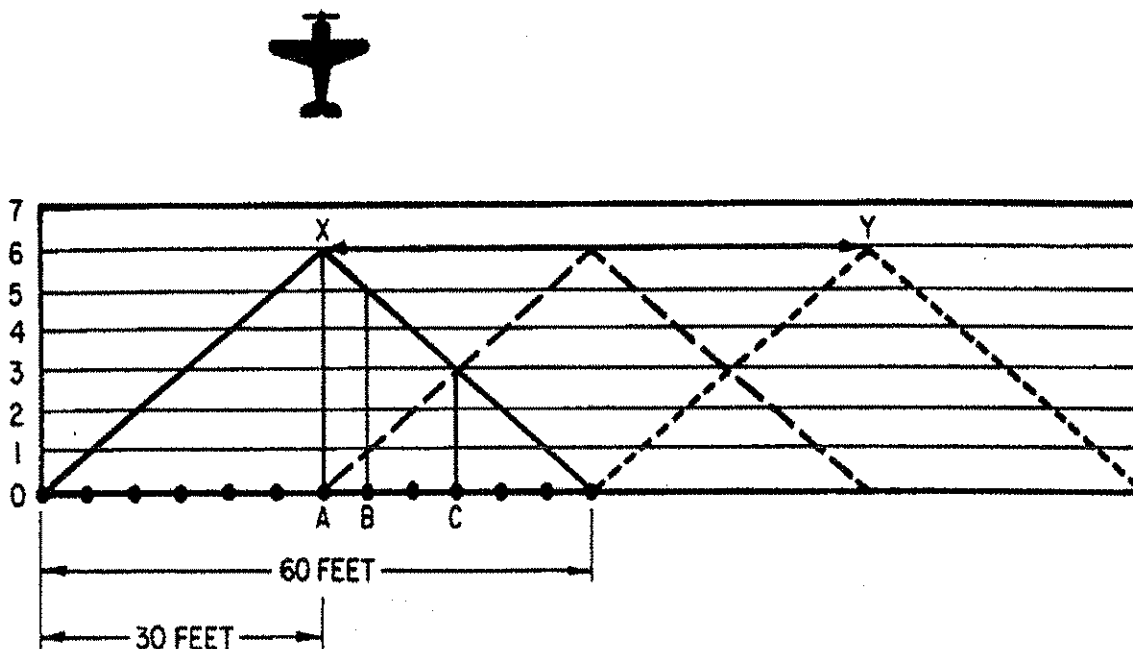
Figure 14. Plot of dry material across the swath.
