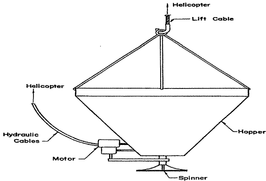
Figure 14. Centrifugal spreader for applying dry materials with rotary wing aircraft
