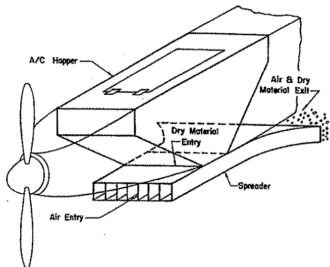
Figure 13. Ram air spreader for applying dry materials.
