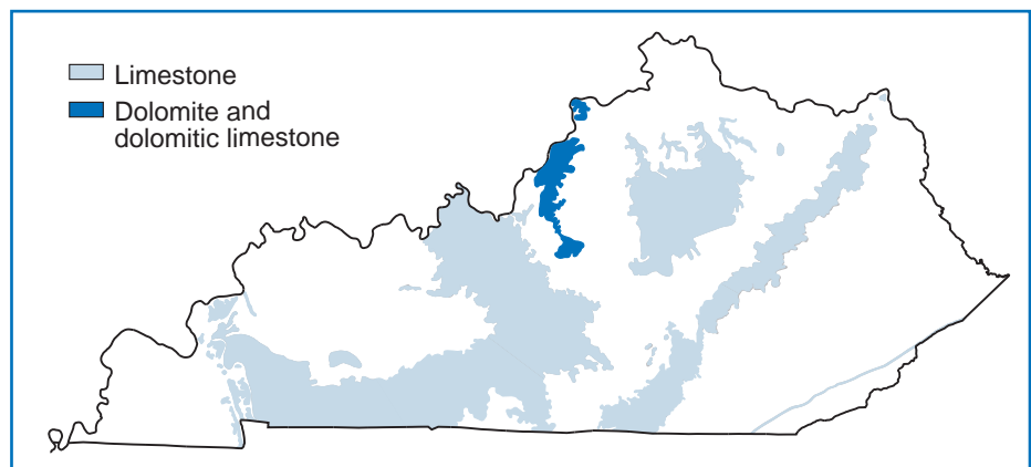
Figure 1. Principal outcrop of limestone and dolomite resources in Kentucky.
