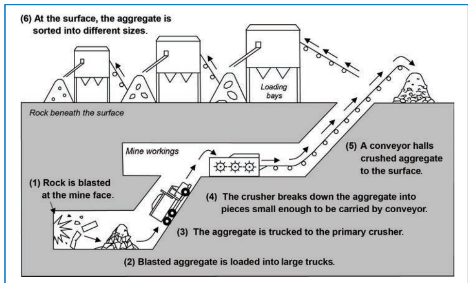
Figure 2. Aggregate mining process
