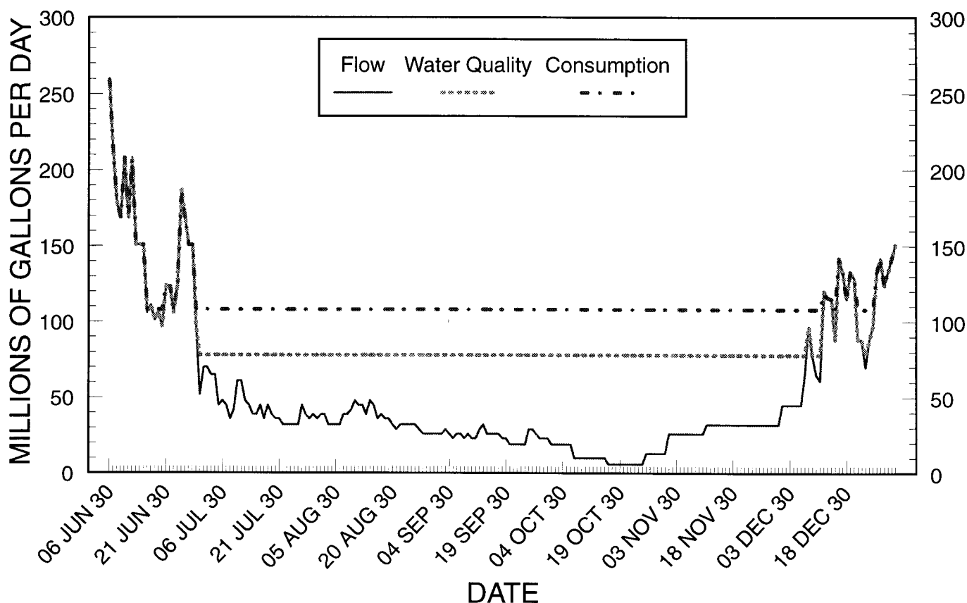
Figure 9. Flow deficit at Lock 10 of the Kentucky River during the drought of 1930.
