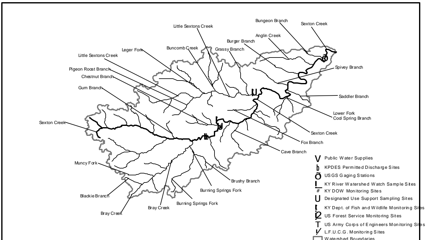
Watershed Features
