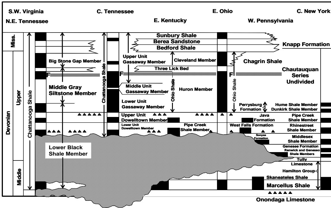
Figure 4. General stratigraphic nomenclature for the Middle and Upper Devonian black shales in the Appalachian Basin. Organic shales are shaded black. "F" indicates the Foerstia Zone. Black triangles indicate major ash beds. Redrawn from de Witt and others (1993). See also Roen and Kepferle, 1993, Plate 2, cross section A-A'.
