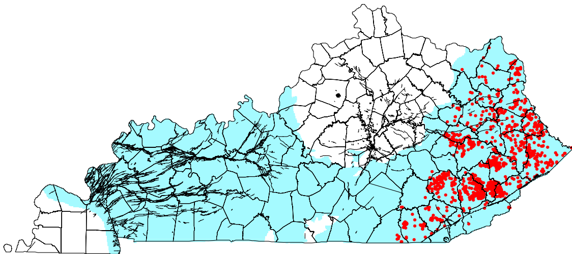
Subsurface distribution of the Devonian shale (blue, shaded) with stratigraphic data points for the Lower Huron Member of the shale.
