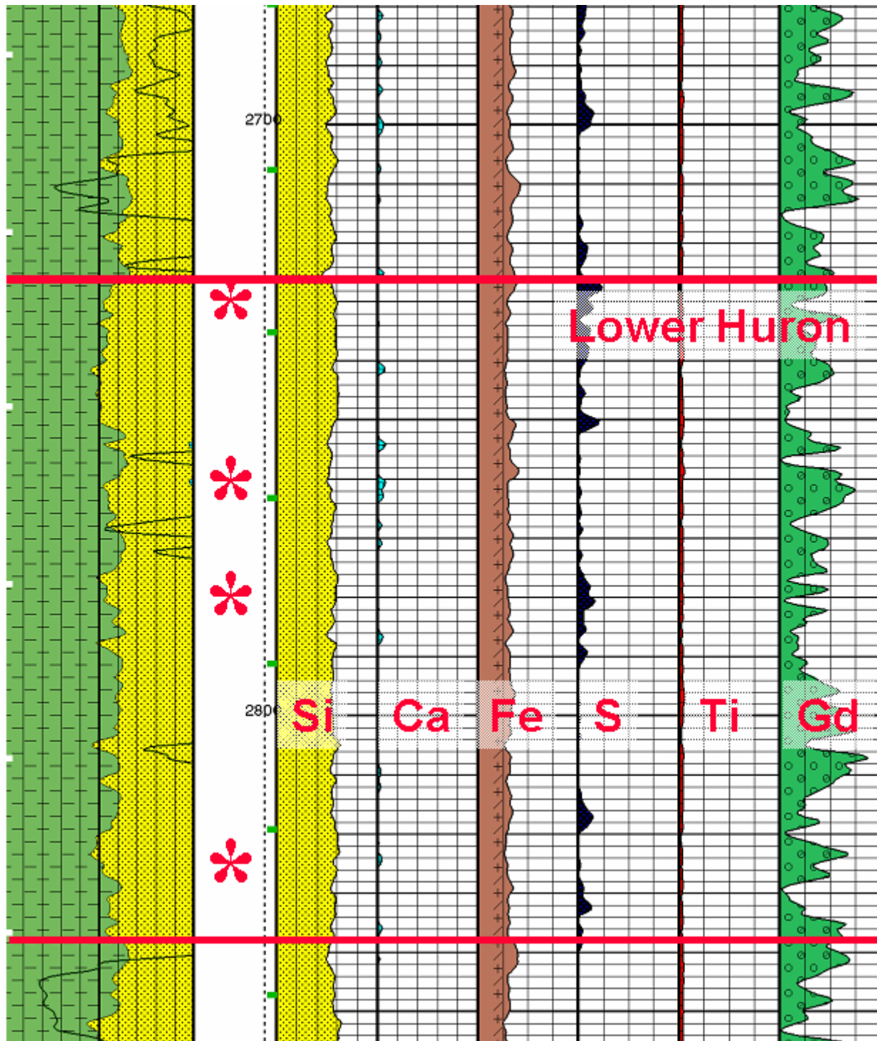
Figure 12. Section of elemental capture spectroscopy log through the Lower Huron section of the Columbia Natural Resources No. 24752 Elk Horn Coal well, Knott County, Ky., showing relative abundance of species related to mineral and lithologic identification. Asterisks denote depths where sidewall cores were recovered.
