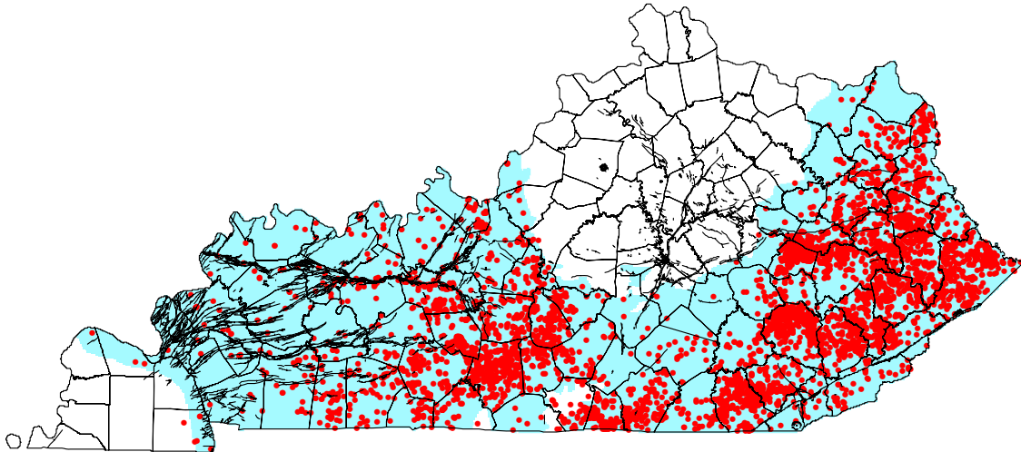
Subsurface distribution of the Devonian shale (blue, shaded) with stratigraphic data points.
