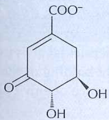
3-Dehydroshikimate
