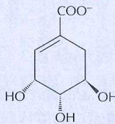
Shikimate
