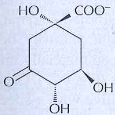
3-Dehydroquinase
