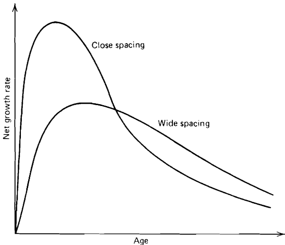
Figure 3.3 An illustration of stand density effects on net growth rate as observed in spacing experiments in even-aged stands.
