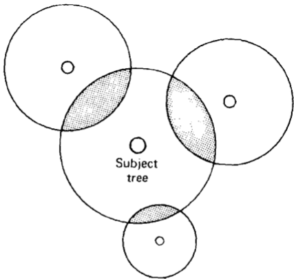
Figure 3.9 An illustration of the competition zone overlap used in the definition of point density measures.
