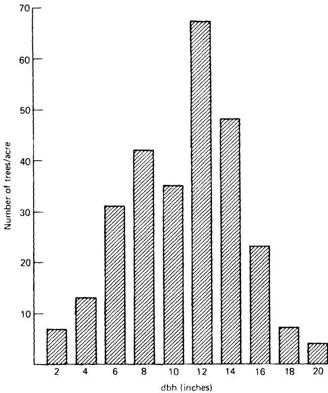
Figure 4.5 Typical diameter distribution for an even-aged stand of upland hardwoods. (After Gingrich, 1978.)
