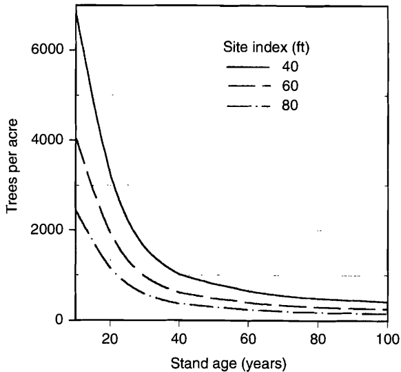
Fig. 10.15. Trees per acre by stand age and oak site index in normally stocked even-aged upland oak stands in the eastern United States. Includes all trees 0.6 inches dbh and larger. (From Schnur, 1937.)
