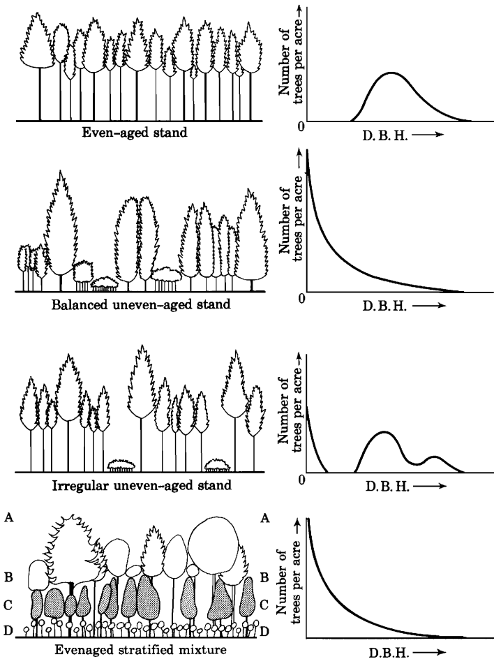
FIGURE 1-3 Typical examples of four different kinds of stand structure, showing appearance of stands in vertical cross section and corresponding graphs of diameter distribution in terms of numbers of trees per unit of area. The trees of the first three stands are all of the same species but the fourth consists of several species but all of the same age.
