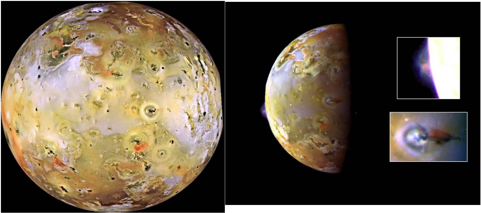
Figure 9- Io
