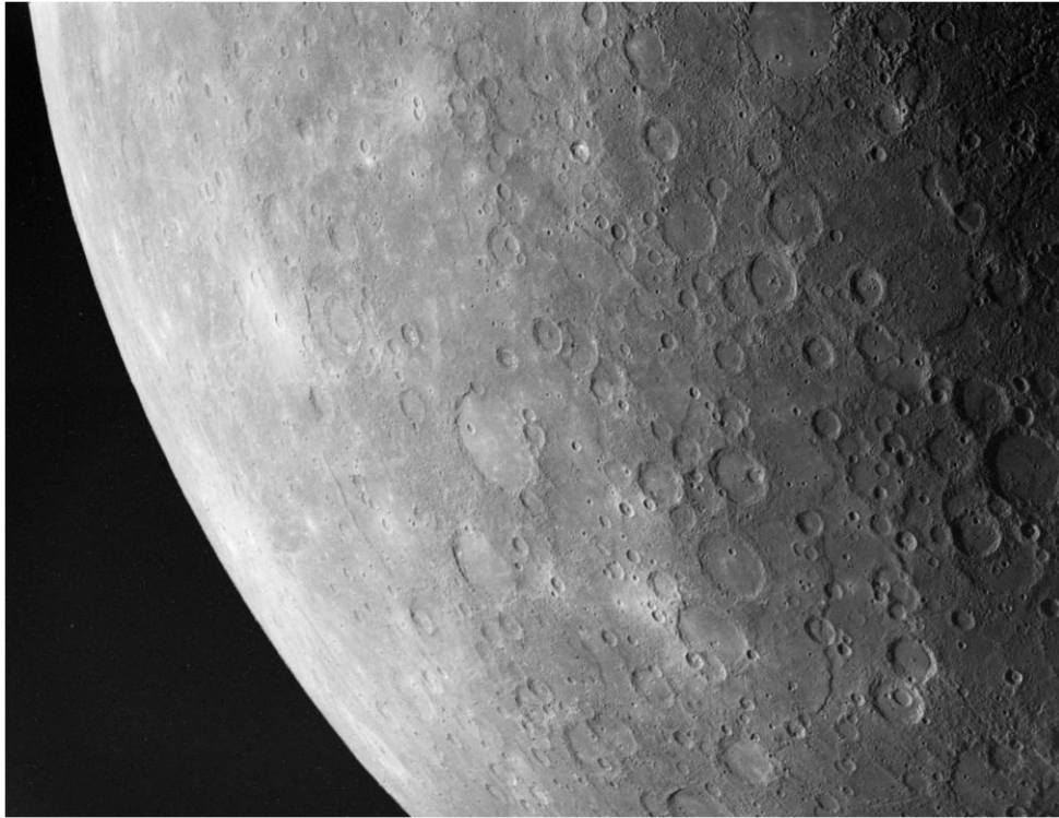
Figure 1: Mercury
