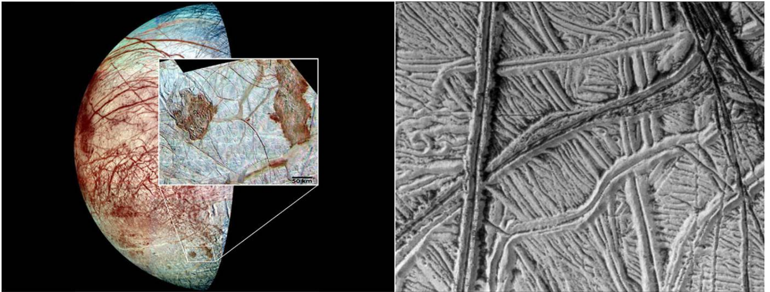
Figure 10- Europa
