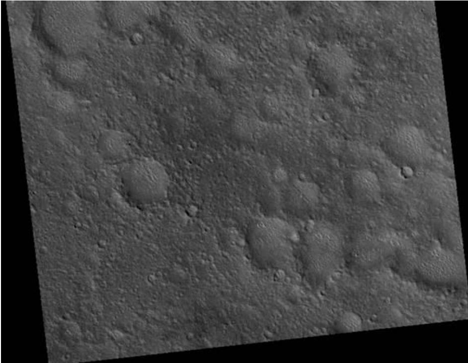
Image 2: Martian Craters
