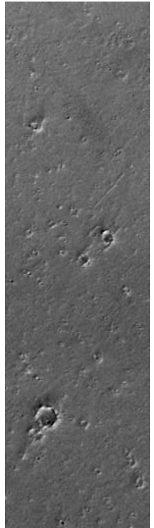
Image 3: Martian Craters
