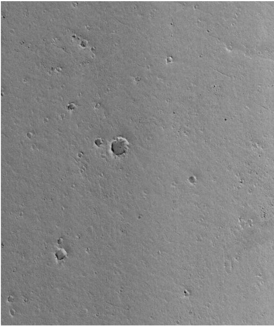
Image 1: Martian Craters
