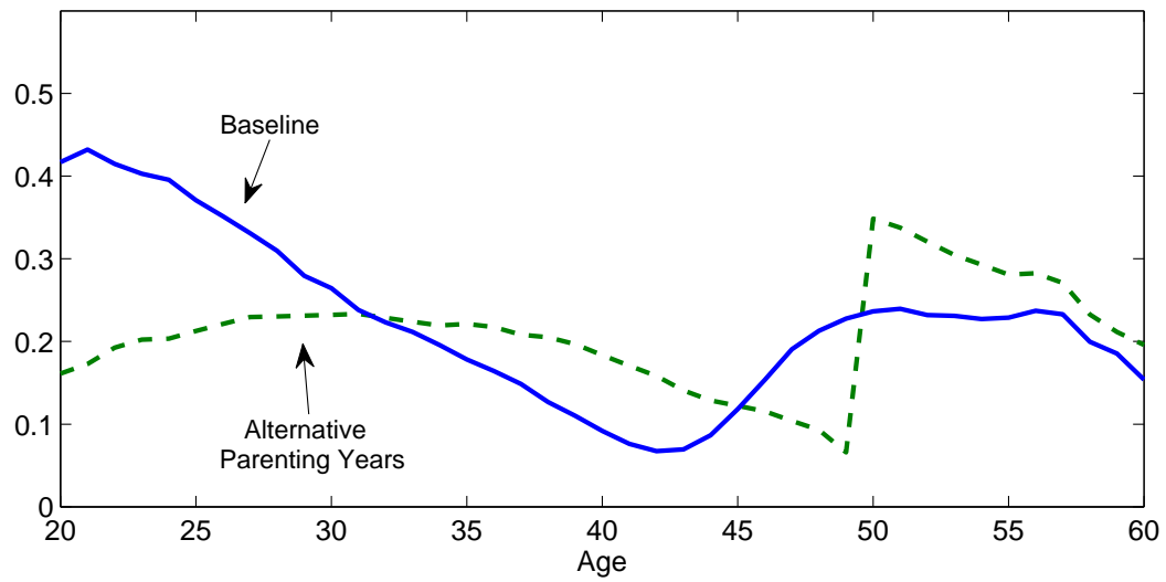
Figure 9: Cross-sectional saving rates by age in 2009 for the baseline demographic change only simulation (solid line) and for the 'Alternative Parenting Years' simulation (dashed line), where parents have a uniform number of dependent children from ages 20-49 and no dependent children thereafter.
