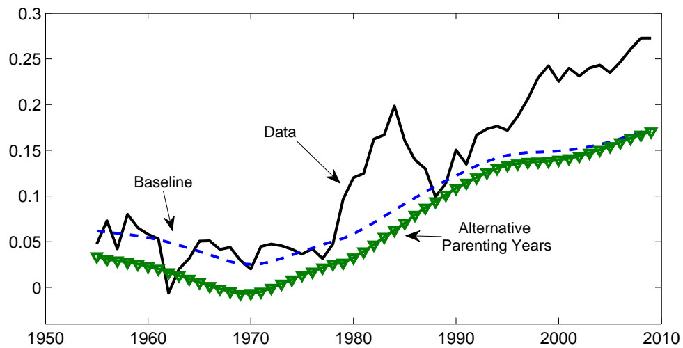
Figure 10: Household saving rates from 1955 to 2009 in the data (solid line), the baseline demographic change only simulation (dashed line), and the ‘Alternative Parenting Years’ simulation, where parents have a uniform number of children from age 20-49 and no dependent children thereafter.
