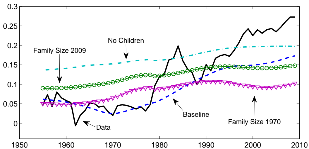
Figure 7: Household saving rates with no children and variations in family size. In the ‘No Children’ simulation, parents do not support dependent children ( \mu = 0 ). In the ‘Family Size’ simulations, the number of dependent children per household is held constant at 1970 and 2009 levels.
