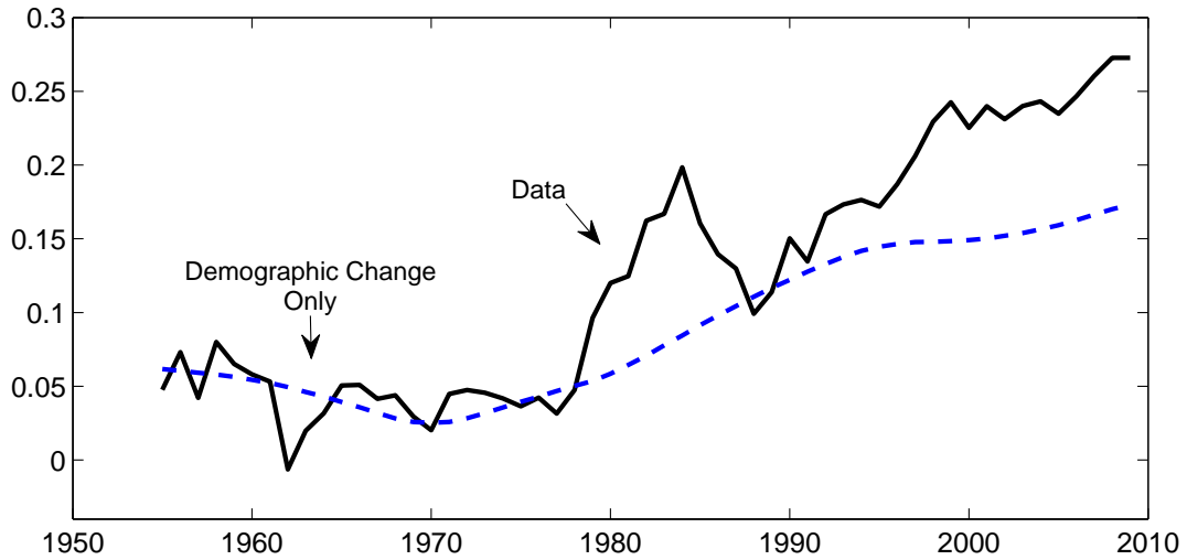
Figure 6: Household saving rates from 1955 to 2009 in the Chinese data and in the model with demographic change only. In the Demographic Change Only simulations wages are fixed in the cross section and r = 0.04 .
