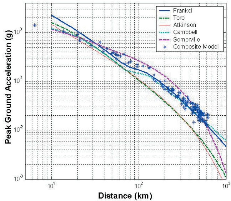
Ground-motion attenuation relationships for M8.0 earthquake
