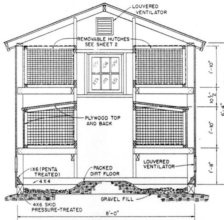
SECTION DOUBLE DECK WIRE FLOOR HUTCH
