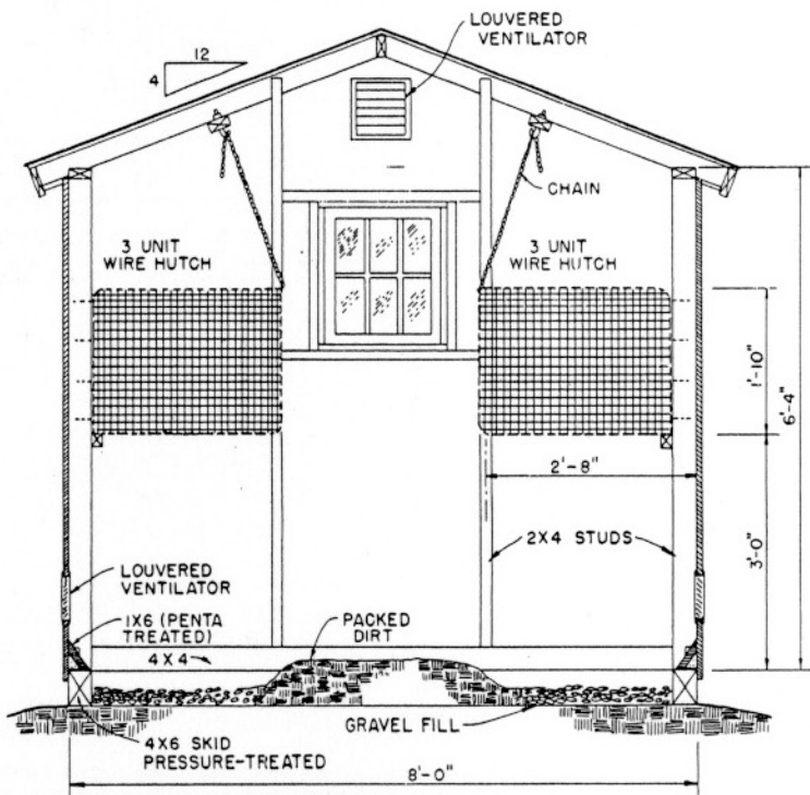
SECTION SINGLE DECK WIRE FLOOR HUTCH
