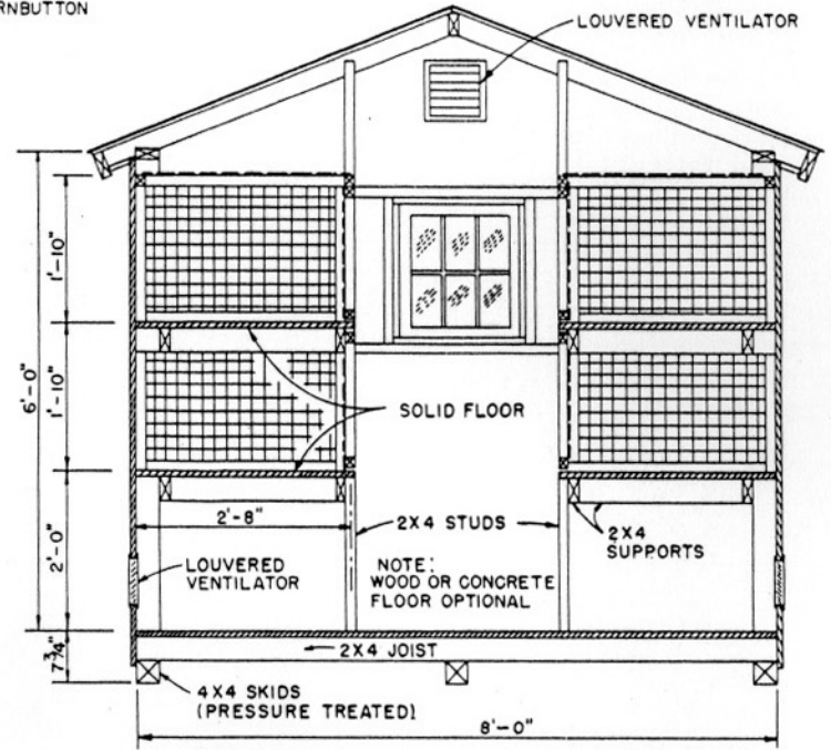
SECTION DOUBLE DECK SOLID FLOOR HUTCH
