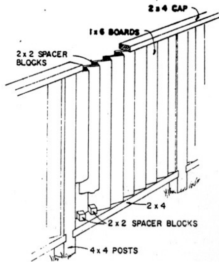
LOUVERED FENCE
