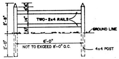
STRETCHER FENCE
