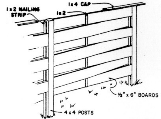
BASKET WEAVE FENCE
