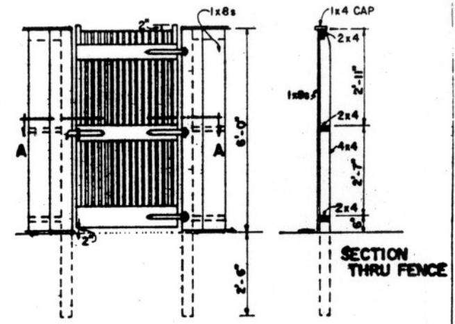
LOUVERED GATE
