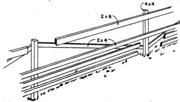
LOW RAIL FENCE
