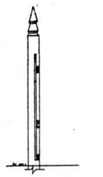
SECTION THRU FENCE
