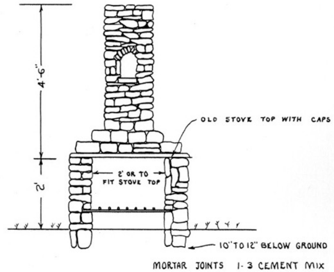
PLAN 3. STONE STOVE
