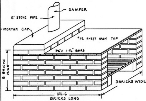
PLAN NO.2. BRICK STOVE
