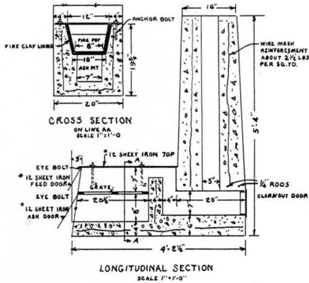
PLAN NO 1 CONCRETE STOVE U.S.O.A.
