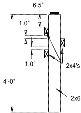
End View Detail
