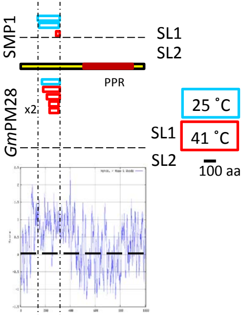
Hydrophilicity Plot / Hopp & Woods
