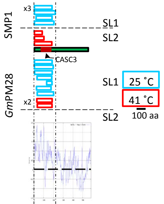
Hydrophilicity Plot / Hopp & Woods
