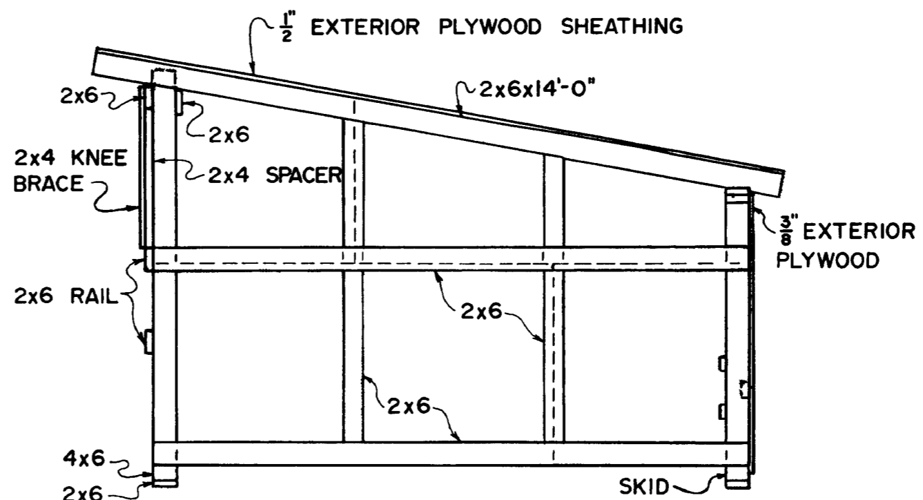
END FRAMING
