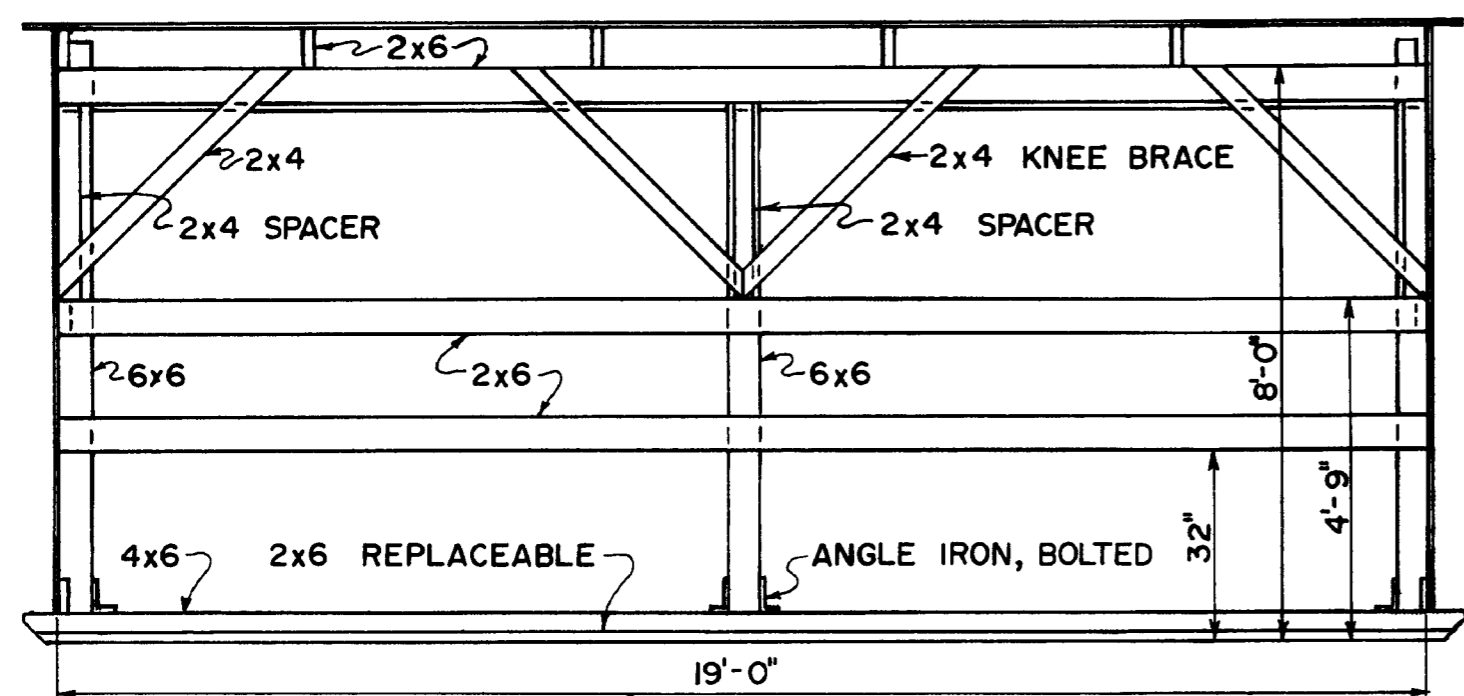
FRONT SIDE FRAMING
