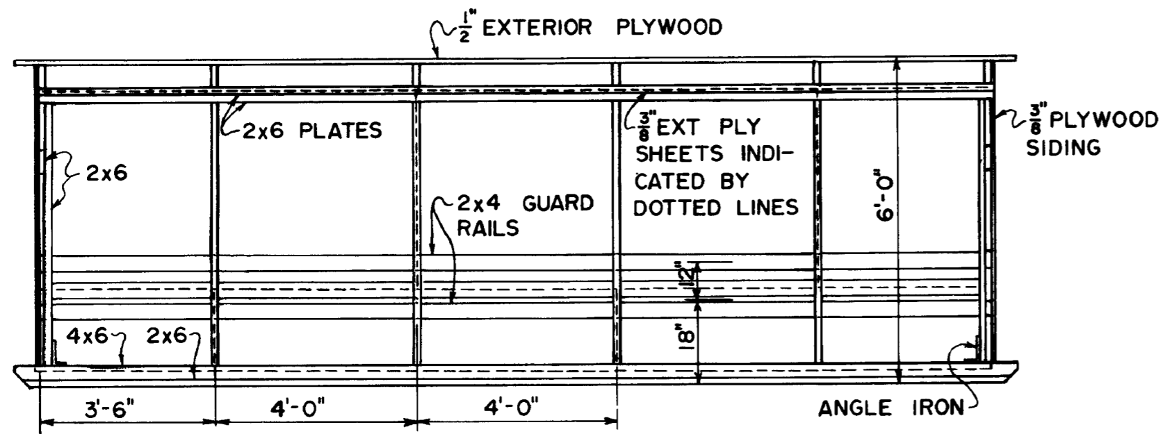
BACK SIDE FRAMING
