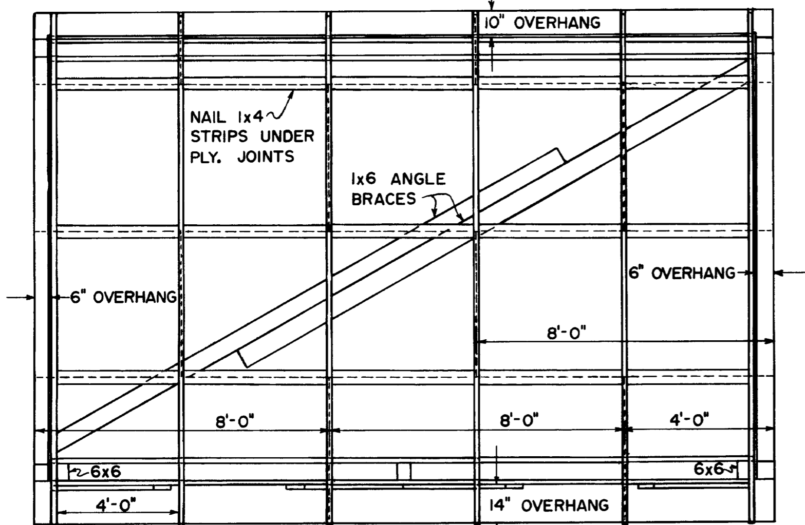
ROOF FRAMING
