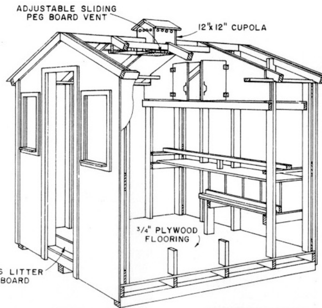
CUTAWAY VIEW OF 8x8' LAYING HOUSE
