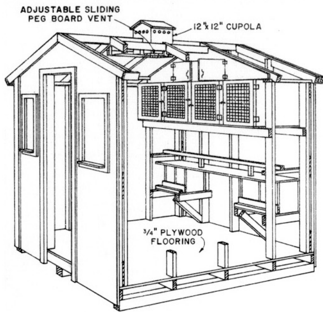
PERSPECTIVE OF CHICKEN HOUSE-BANTAMS
