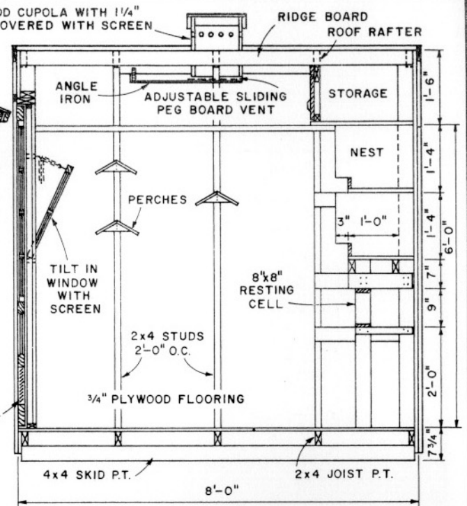
SECTION OF PIGEON HOUSE
