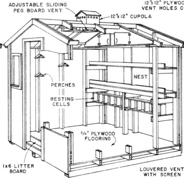
PERSPECTIVE OF PIGEON HOUSE
