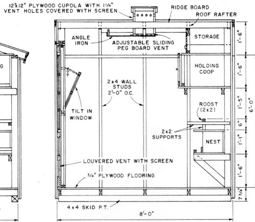
SECTIONS OF CHICKEN HOUSE-BANTAMS
