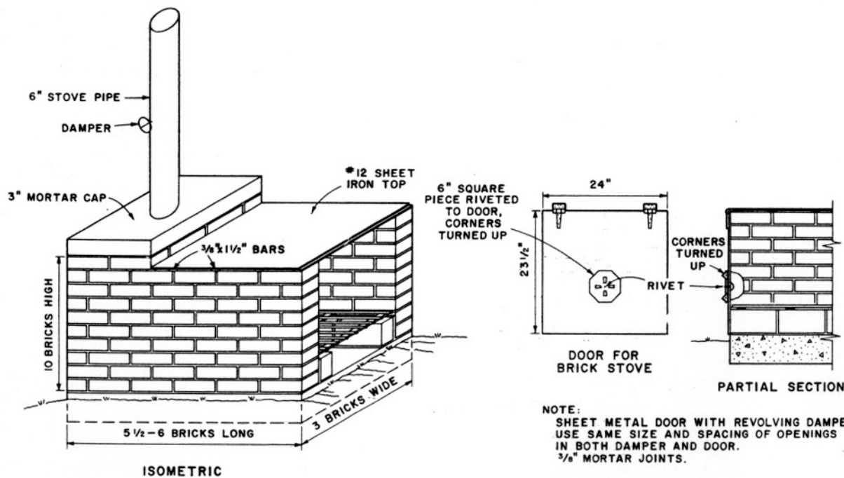
PLAN NO. 2 BRICK STOVE
